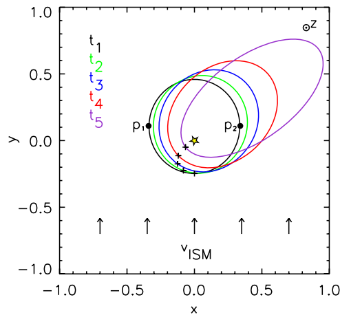
Figure 10. Orbital evolution of a test particle in the x - y plane under the effect of neutral gas drag. Five time periods separated by a fixed number of orbits are shown. The grain begins with its star-pericenter (Runge-Lenz) vector anti-aligned with the incoming interstellar flow, directed along the positive y -axis, and its angular momentum vector aligned with the z -axis (out of the page). The ISM flow decelerates the grain on one leg (e.g., point p_1 ) and accelerates it on the other (e.g., point p_2 ), causing the Runge-Lenz vector to rotate. The grain's periastra at each successive time is shown by a cross to illustrate this effect.
