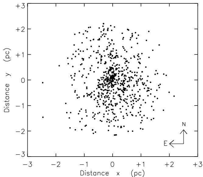
FIG. 1.—Positions in the sky of the 705 ONC stars with 67% membership probability (from Hillenbrand 1997). The x - and y -axes are oriented in the directions of right ascension and declination, respectively, and a distance of 480 pc is assumed.
