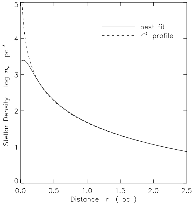
FIG. 3.—Reconstructed, three-dimensional density of stars, compared to a r^{-2} profile (dashed curve). The inward falloff in the reconstructed density is not real but reflects incompleteness of the optical sample in the crowded central region.
