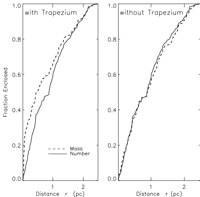
Fig. 5.—Comparison of the distributions of stellar mass and number as a function of radius. Left : When the Trapezium is included, the mass curve immediately climbs higher than the stellar number. Right : Without the Trapezium, the two distributions are nearly identical, indicating uniformity of the stellar mass spectrum.
