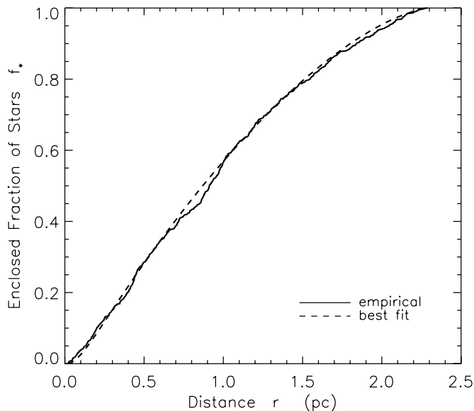
FIG. 2.—Projected number density of stars. The fraction of the total stellar population of 705 stars is shown as a function of projected radius. The dashed curve is a smooth fit to the data.
