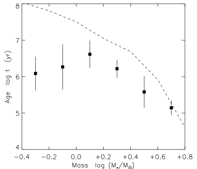
FIG. 9.—Pre-main-sequence stellar age as a function of mass. This plot was constructed in a manner analogous to Fig. 8. The dashed curve represents the total contraction time to the zero-age main sequence at each mass value.
