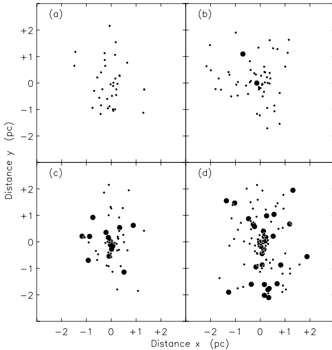
FIG. 7.—Positions of ONC stars (from the sample of 244) that were born (a) more than 5 Myr ago, (b) from 2 to 5 Myr ago, (c) from 1 to 2 Myr ago, and (d) more recently than 1 Myr ago. The smaller filled circles denote stars with M_* < 2 M_\odot , while the larger ones are for 2 M_\odot < M_* < 8 M_\odot .
