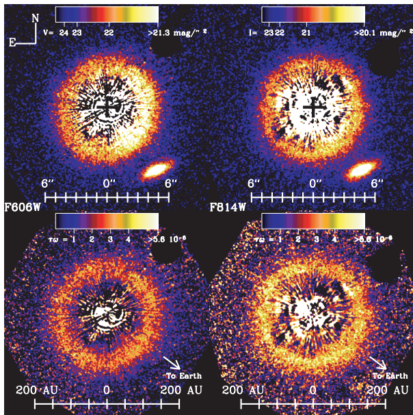
FIG. 1.—Disk around the G2 V star HD 107146. Top left : F606W filter (broad V); top right : F814W filter (broad I). To obtain these images, a reference PSF (HD 120066) was normalized to, aligned with, and subtracted from the coronagraphic images of HD 107146. The 3''.0 spot in the upper right-hand corner has been masked out. Bottom : Maps of the scattering optical depth \tau_{\omega} (the product of the total optical depth times the albedo), obtained by de-projecting the disk (assuming an inclination of 25^\circ from face-on), multiplying by the distance squared from the stellar position, correcting for forward scattering, and dividing by the stellar flux. Bottom left : F606W filter; bottom right : F814W filter. Note that the bottom row images have the same color scale but that the top row ones do not. FITS versions of these images are available as a gzipped tar file in the electronic edition of the Journal.
