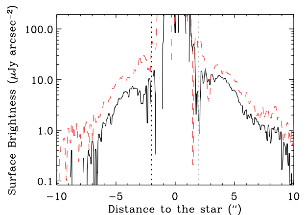
FIG. 2.—Surface brightness as a function of distance, obtained by taking the median of the flux in rectangular boxes 2'' wide (centered in the stellar position) by 0''.125 long. The measurements are taken along a path with a position angle of 58^\circ (the disk's minor axis). Positive displacements are toward the southwest. The thick-black (red-dashed) line is the trace in the F606W (F814W) band. The dotted lines are positioned at 2'' from the star. This profile suggests that subtraction residuals dominate beyond 6''.5 , at the level of \sim 1 \mu\text{Jy arcsec}^{-2} ; 10 \mu\text{Jy arcsec}^{-2} ; 10 \mu\text{Jy arcsec}^{-2} correspond to V = 21.48 or I = 20.95 .
