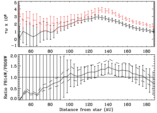
FIG. 3.— Top : Median \tau\omega as a function of distance from the star, obtained in a series of annuli 0".14 wide, measured from the bottom panels of Fig. 1. The solid line is the F606W observation ( g_{\text{F606W}} = 0.3 \pm 0.1 ). The red-dashed line is the F814W observation ( g_{\text{F814W}} = 0.2 \pm 0.1 ). The error bars indicate the range of values obtained if the standard PSF is oversubtracted or under-subtracted by 1%. Bottom : Ratio of (\tau\omega)_{\text{F814W}} to (\tau\omega)_{\text{F606W}} , as a function of distance from the star. As above, the error bars show the dependence on errors in the normalization. The dashed lines indicate the dependence of the ratio on the value of g : the top dotted line is obtained assuming g_{\text{F606W}} = 0.2 and g_{\text{F814W}} = 0.3 , and the bottom one is obtained assuming g_{\text{F606W}} = 0.4 and g_{\text{F814W}} = 0.1 . These choices produce extremal ratios.
