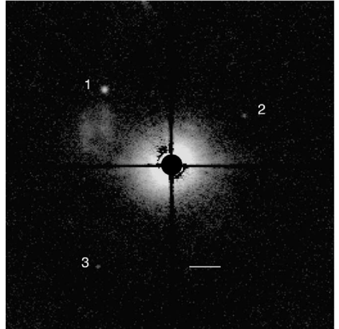
FIG. 2.— R -band coronagraphic image of 55 Cnc after PSF subtraction. North is up, east is left, and the bar represents 10". A 6".5 diameter, hard-edged occulting spot is supported by four wires at the telescope focal plane. Spurious instrumental scattered light is evident as an extended feature northeast of 55 Cnc and south of source 1.
