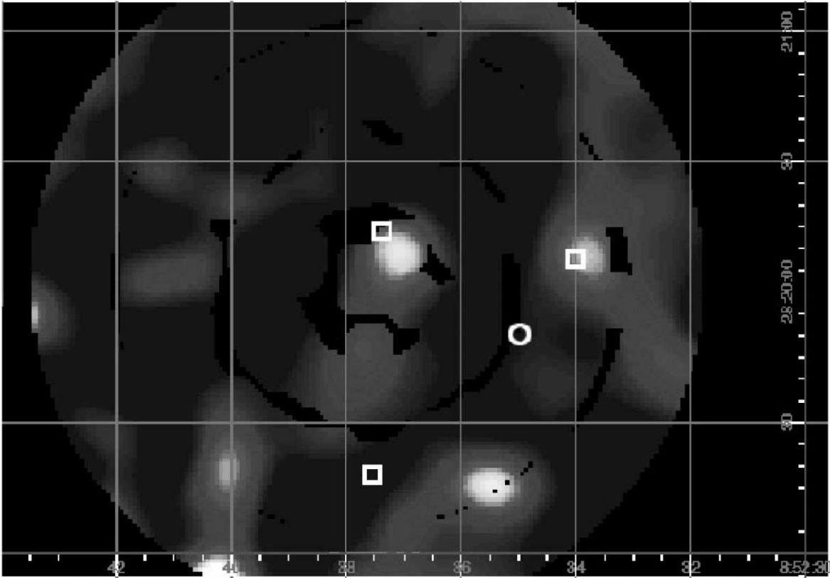
FIG. 1.—JCMT/SCUBA 850 \mu\text{m} map of the region surrounding 55 Cnc. The star's position is marked by the white circle. Positions of optical R -band sources are marked by white boxes. The map is produced from photometry observations at two different pointings. Each individual pointing produces a map with concentric rings. Even with two separate pointings, combined with the effects of sky rotation, a fully sampled map is not produced, and hence residual holes are evident. [See the electronic edition of the Journal for a color version of this figure.]
