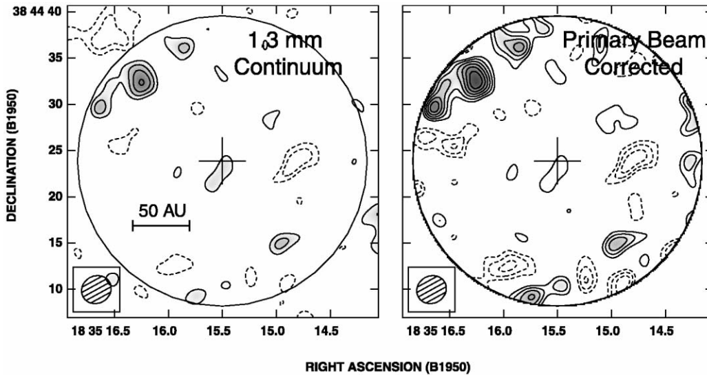
FIG. 1.— Left : Aperture synthesis image of 1.3 mm emission from Vega ( \alpha Lyrae). Contours are at 1\sigma intervals of 0.5 mJy, starting at the 2\sigma level. The position of Vega is marked with a plus sign; the half-power circumference of the primary beam of the 10.4 m telescopes is shown as a circle. The synthesized beam, 3''.3 \times 2''.9 FWHM at P.A. = 119^\circ , is represented by a hatched circle. Right : Same as the left panel, except that compensation has been made for the radial falloff in intensity due to the primary-beam pattern.
