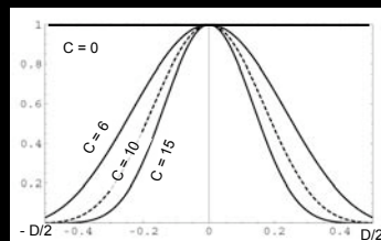
3 different apodized apertures
