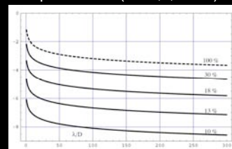
Attenuated solar limb for 4 apodizations ( c = 4, 6, 8 \text{ \& } 10 )
