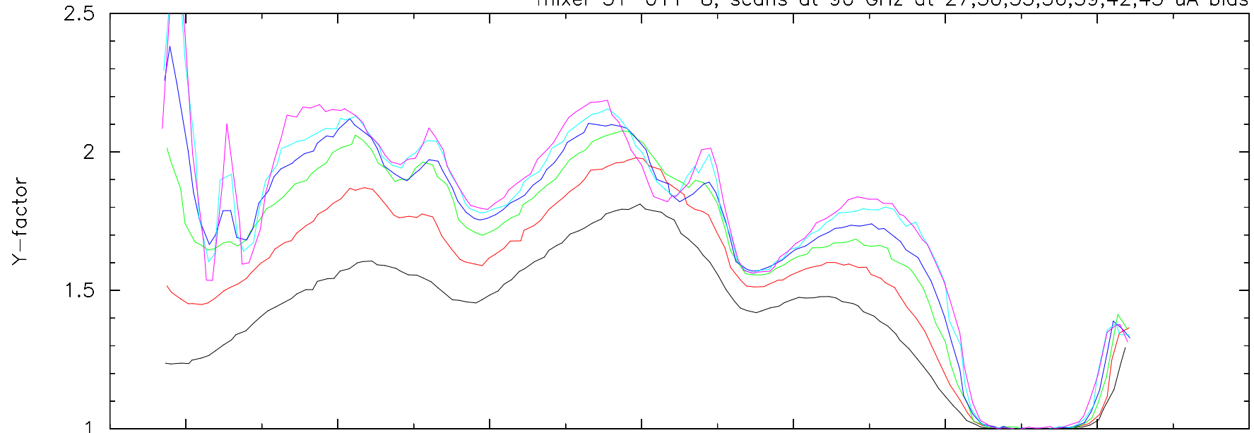
mixer 31-011-8; scans at 90 GHz at 27,30,33,36,39,42,45 uA bias
