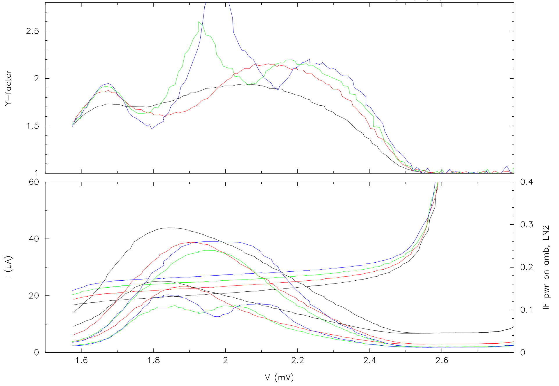
mixer 31-015A-1; scans at 260 GHz; 21,23,25,27 uA at 2.0 mV
