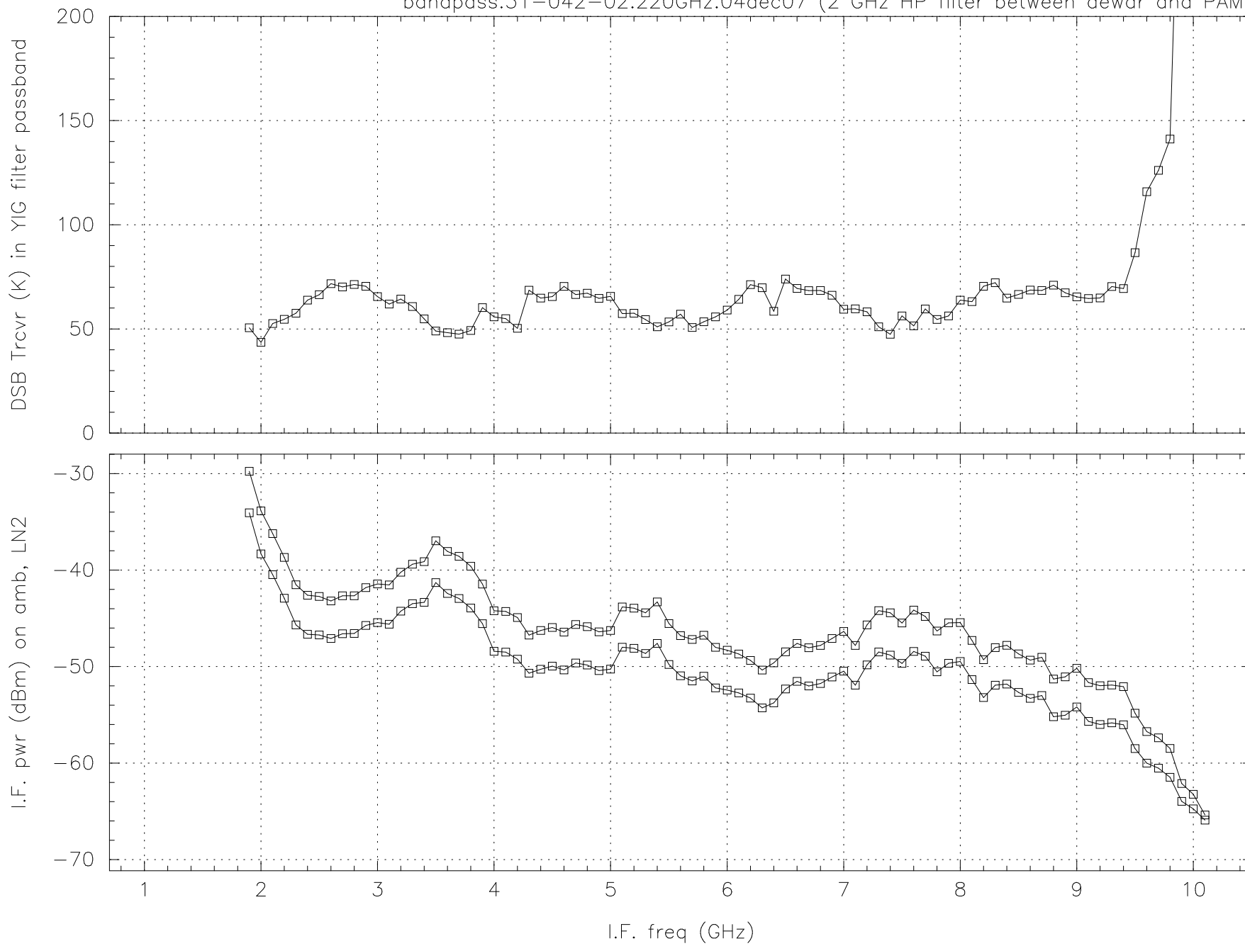
bandpass.31-042-02.220GHz.04dec07 (2 GHz HP filter between dewar and PAM)
