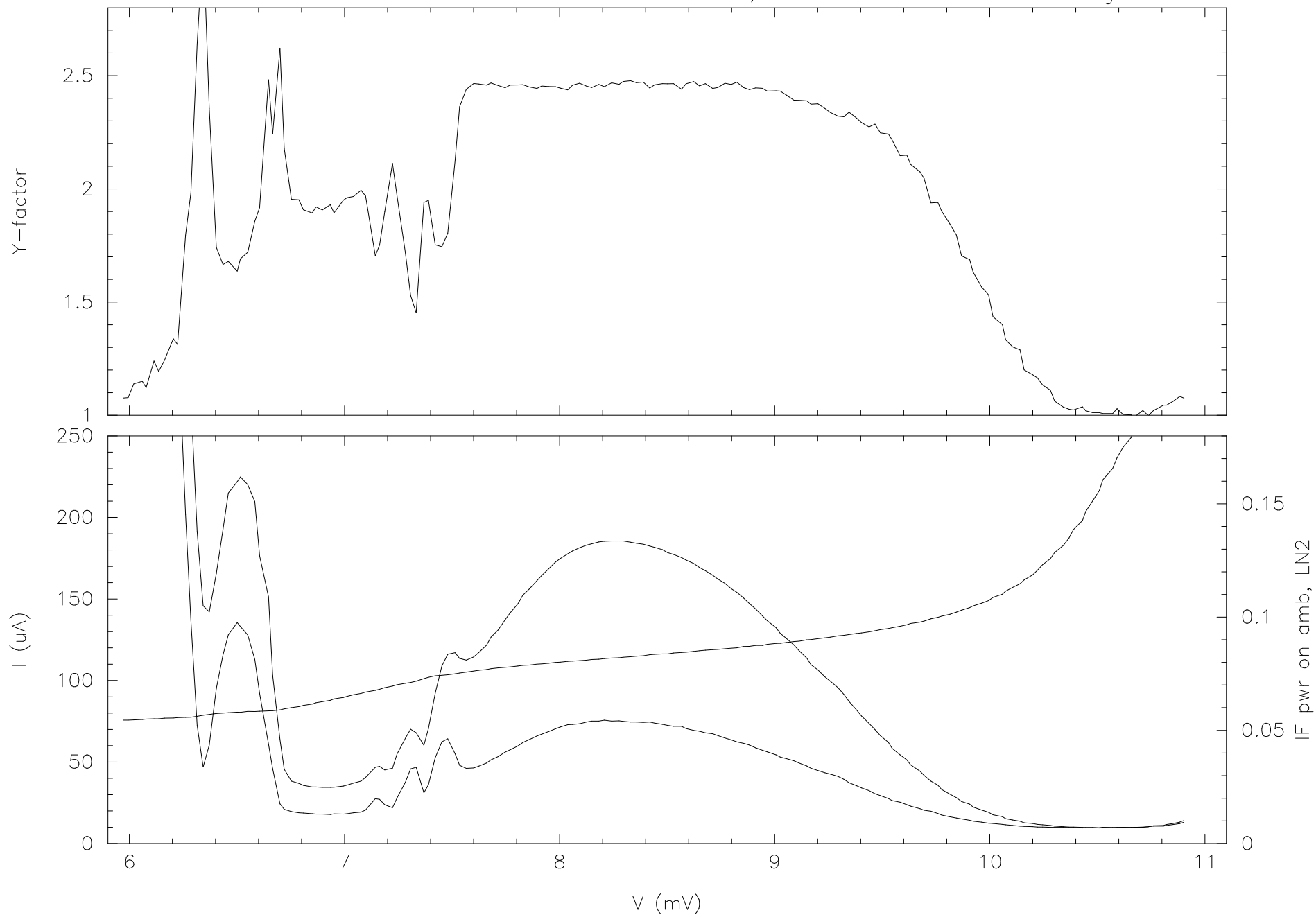
mixer 31-042-02; scans at 220 GHz with 0 mA magnet current
