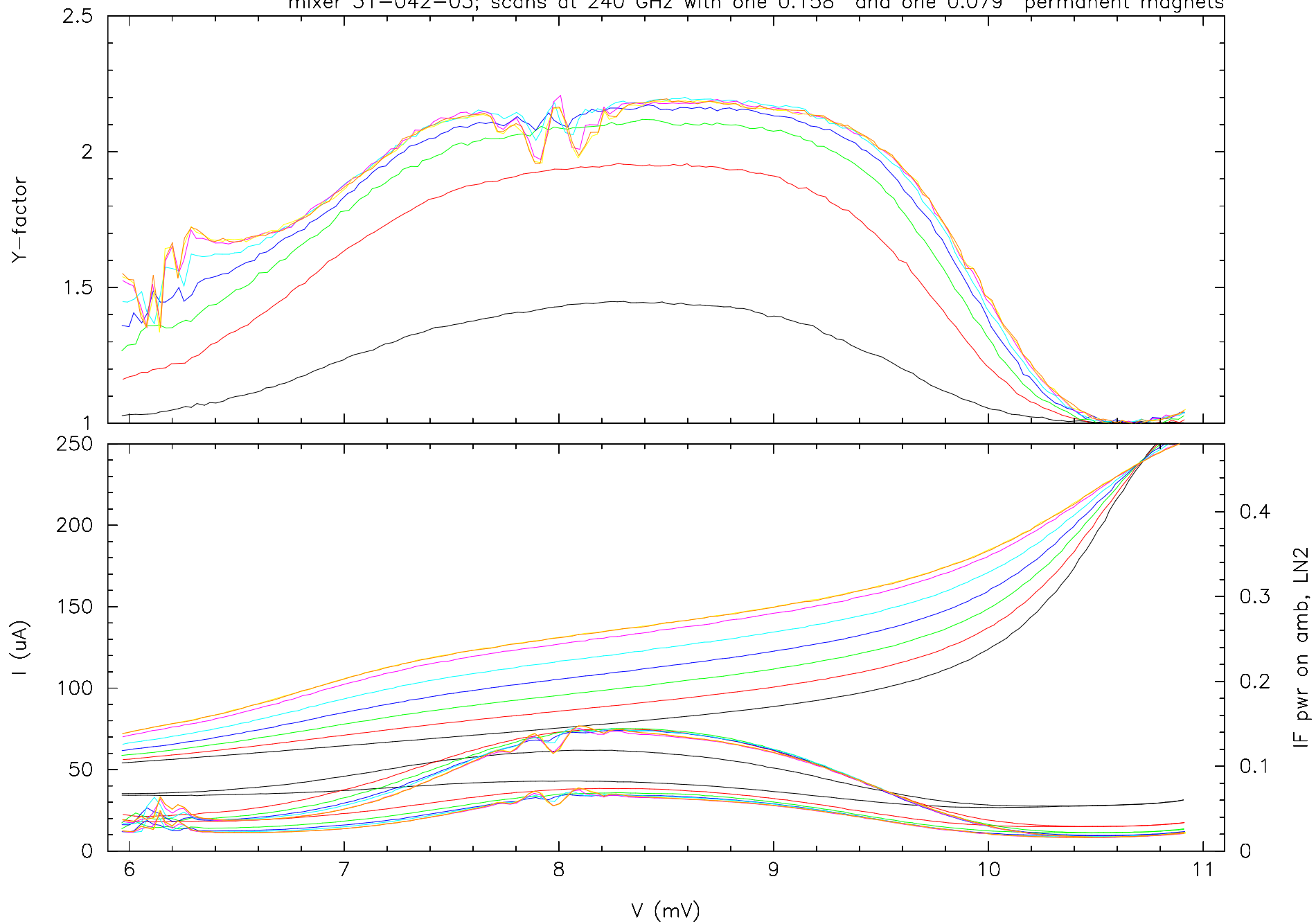
mixer 31-042-03; scans at 240 GHz with one 0.158" and one 0.079" permanent magnets
