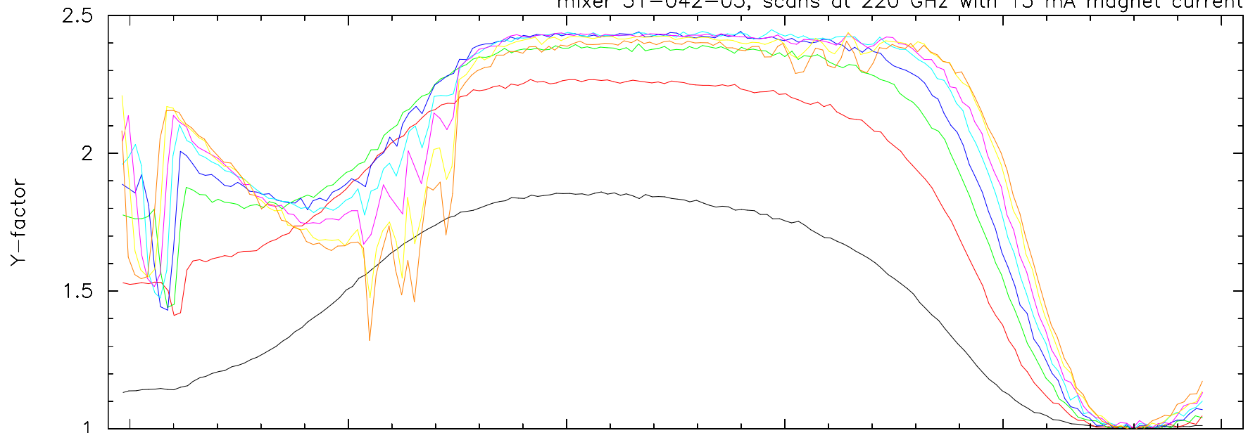
mixer 31-042-03; scans at 220 GHz with 15 mA magnet current
