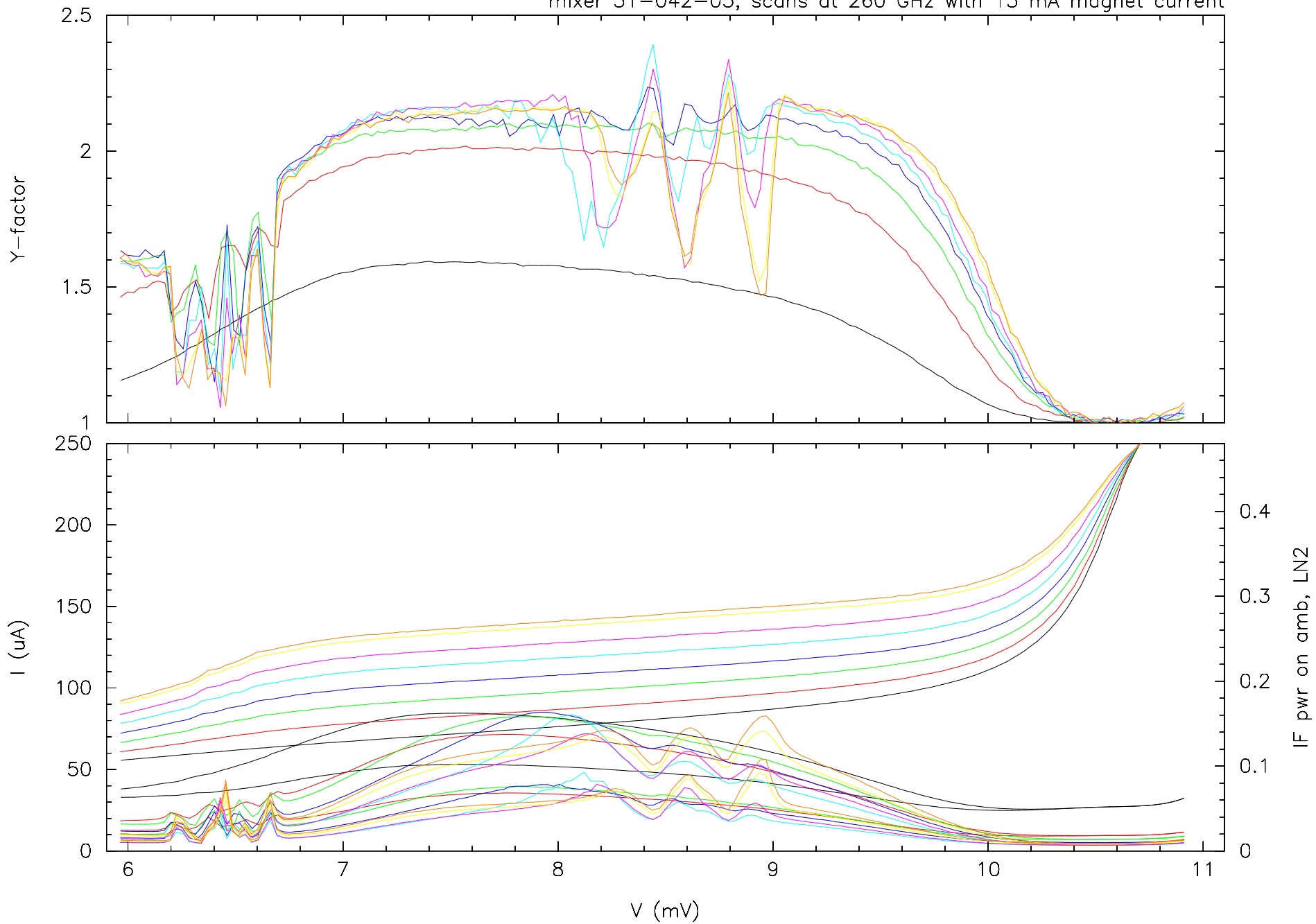
mixer 31-042-03; scans at 260 GHz with 15 mA magnet current
