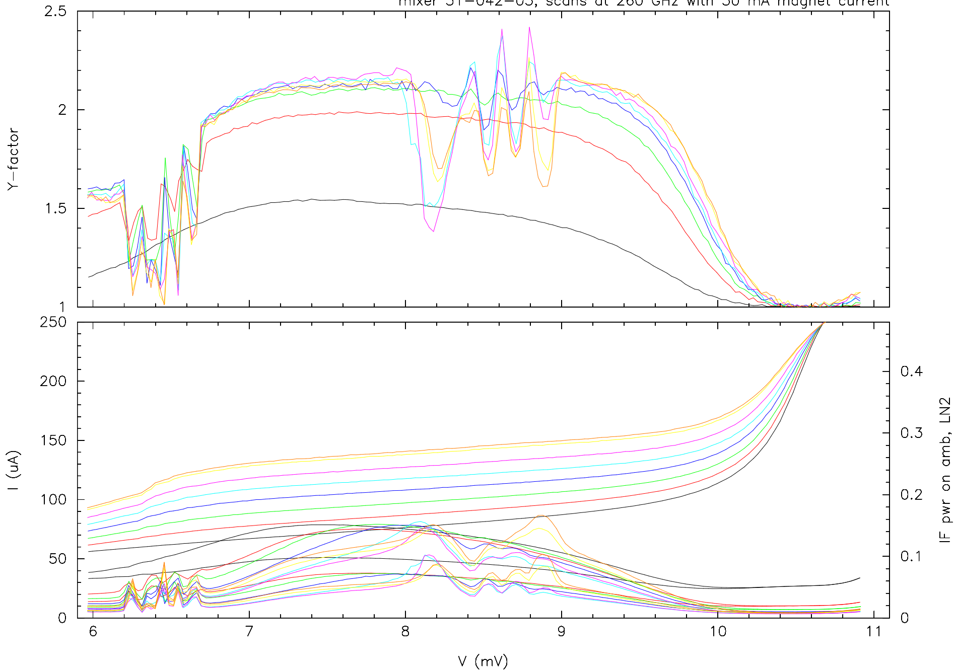
mixer 31-042-03; scans at 260 GHz with 30 mA magnet current
