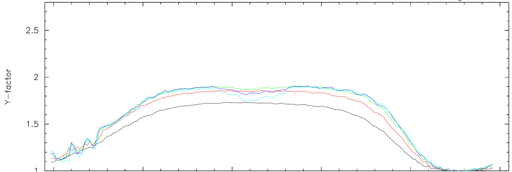
mixer 31-042-03; scans at 250 GHz with 45 mA magnet current
