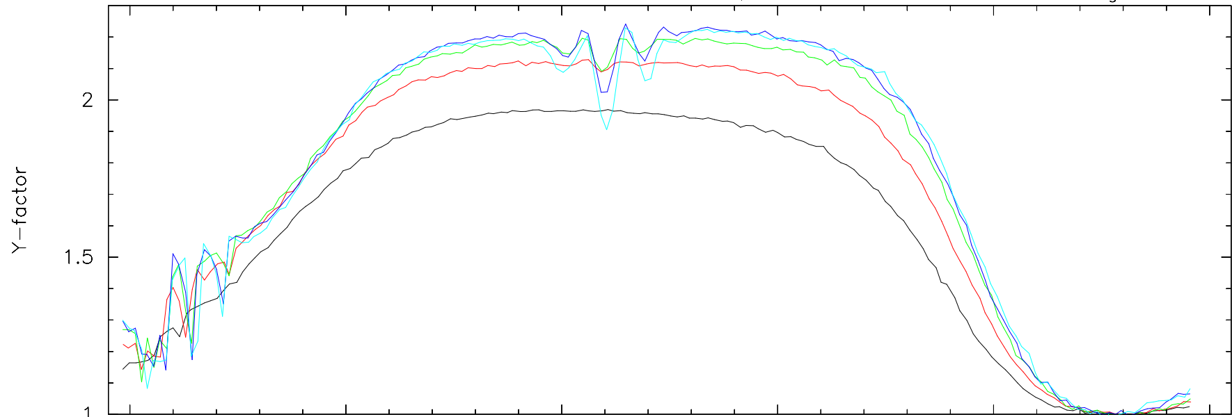
mixer 31-042-03; scans at 250 GHz with 36 mA magnet current
