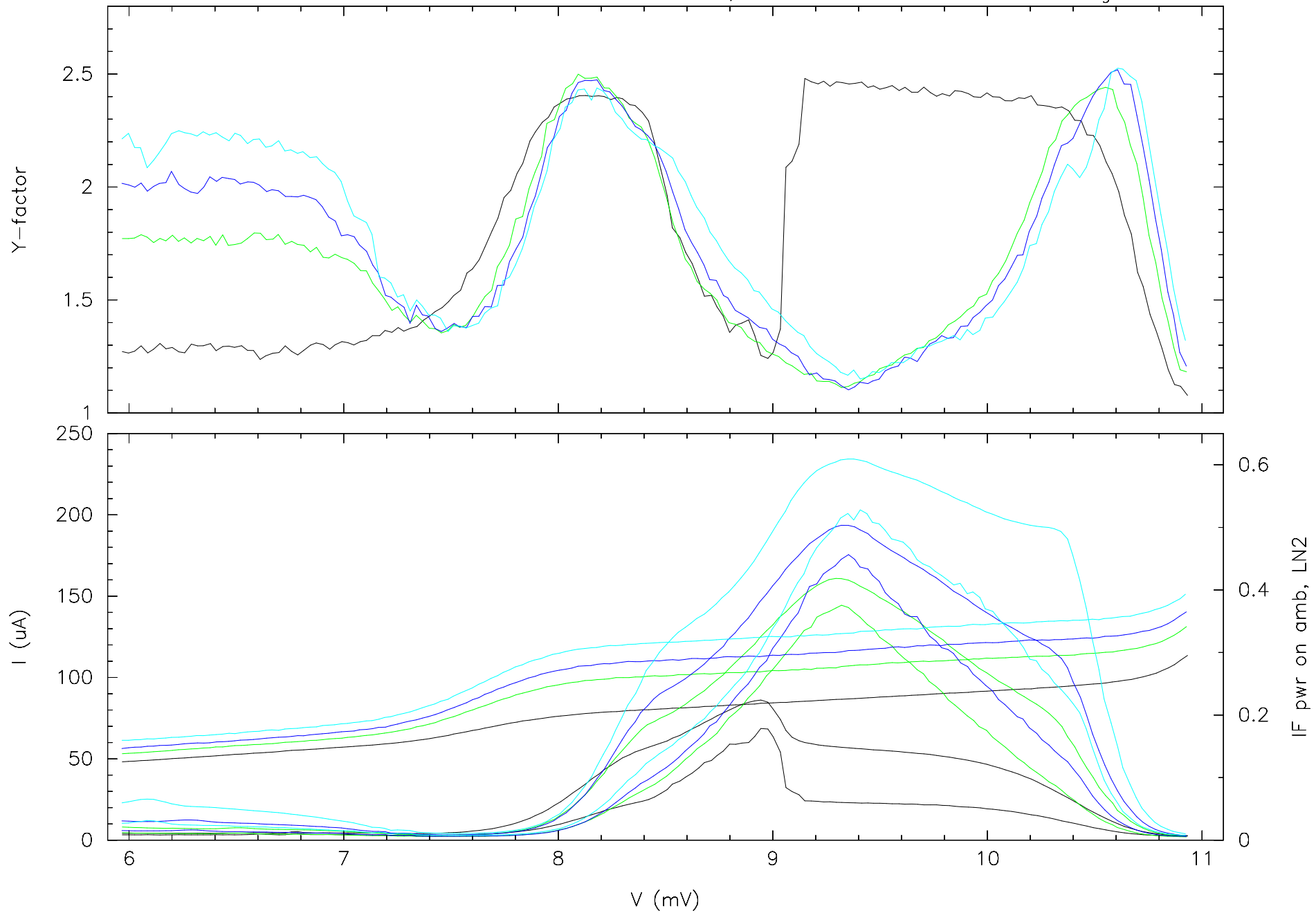
mixer 31-042-04; scans at 220 GHz with 9.8 mA magnet current
