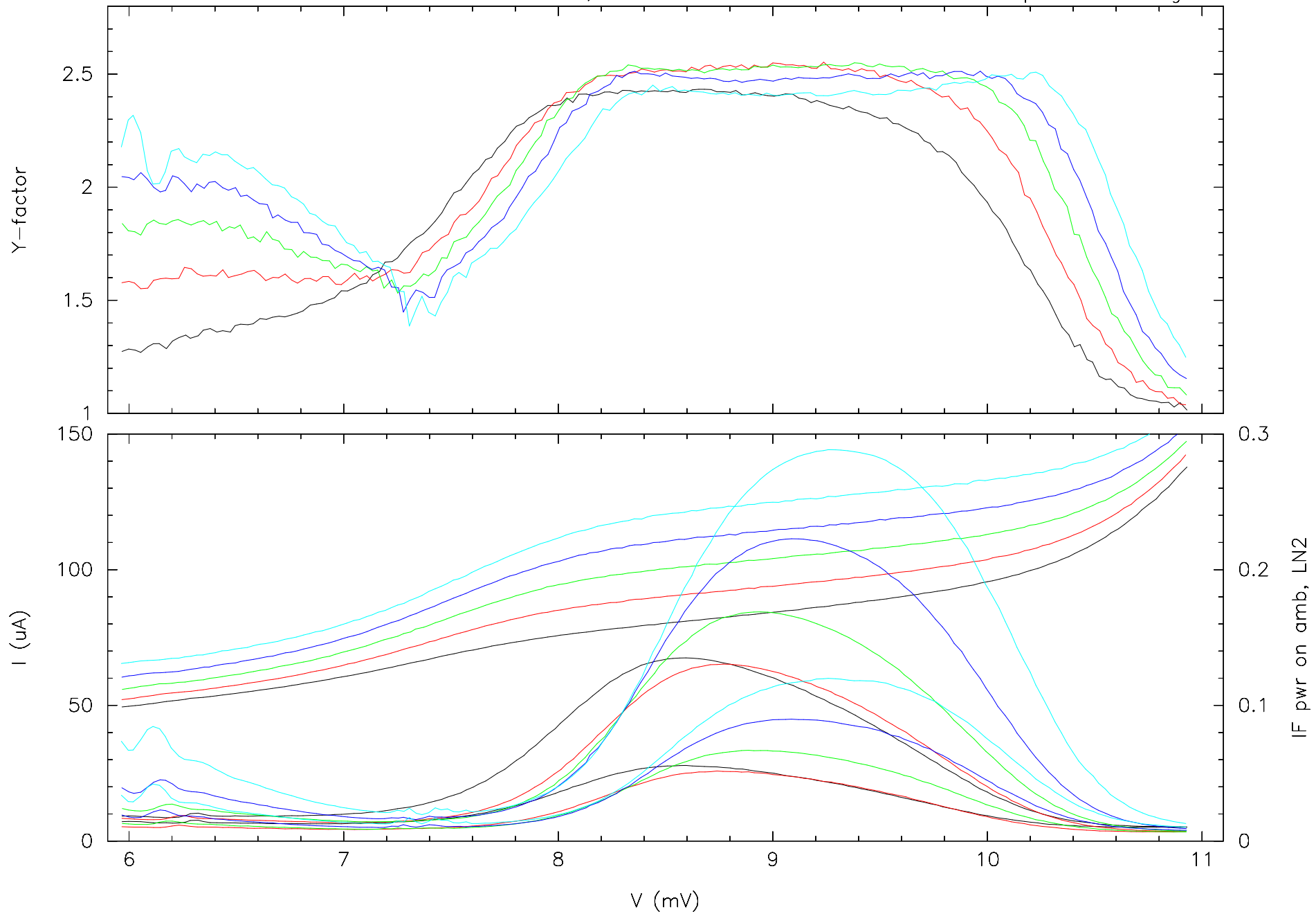
mixer 31-042-04; scans at 220 GHz with two 0.158" diam permanent magnets
