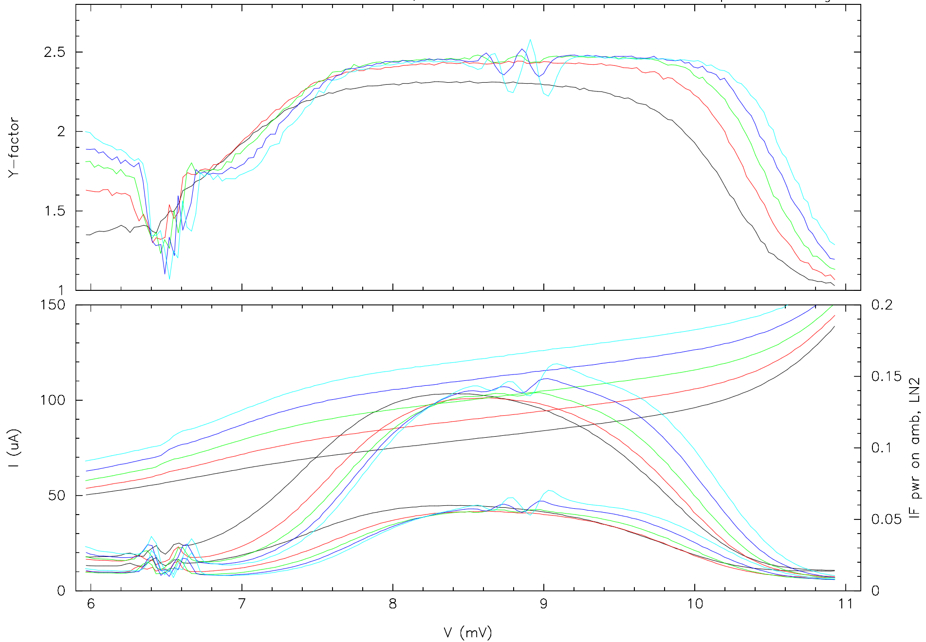
mixer 31-042-04; scans at 260 GHz with two 0.158" diam permanent magnets
