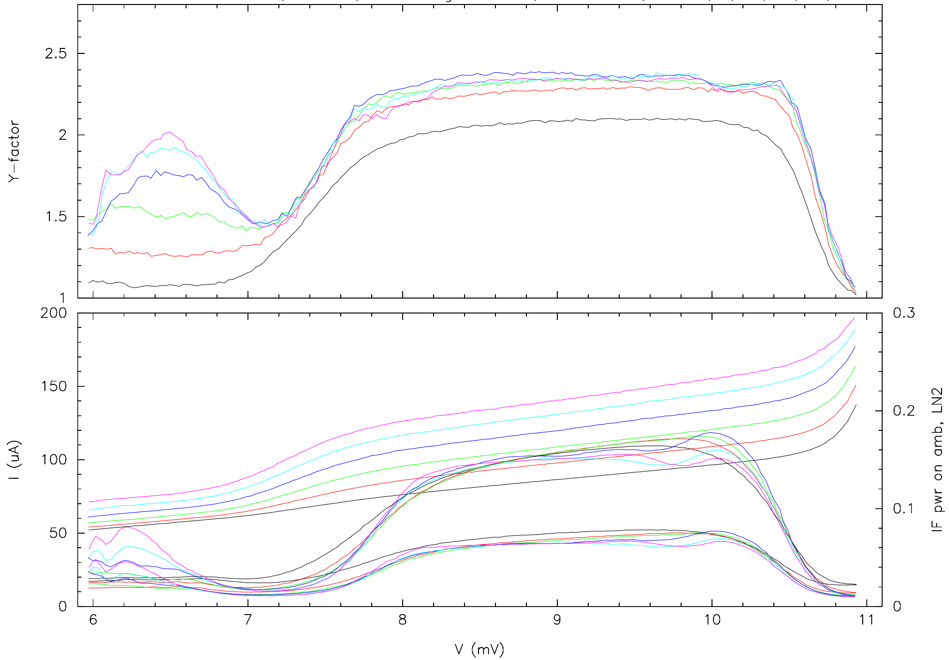
mixer 31-042-05, 240 GHz, 20 mA magnet current, 2 GHz HP filt; bias 80,90,100,110,120,130 \mu\text{A}
