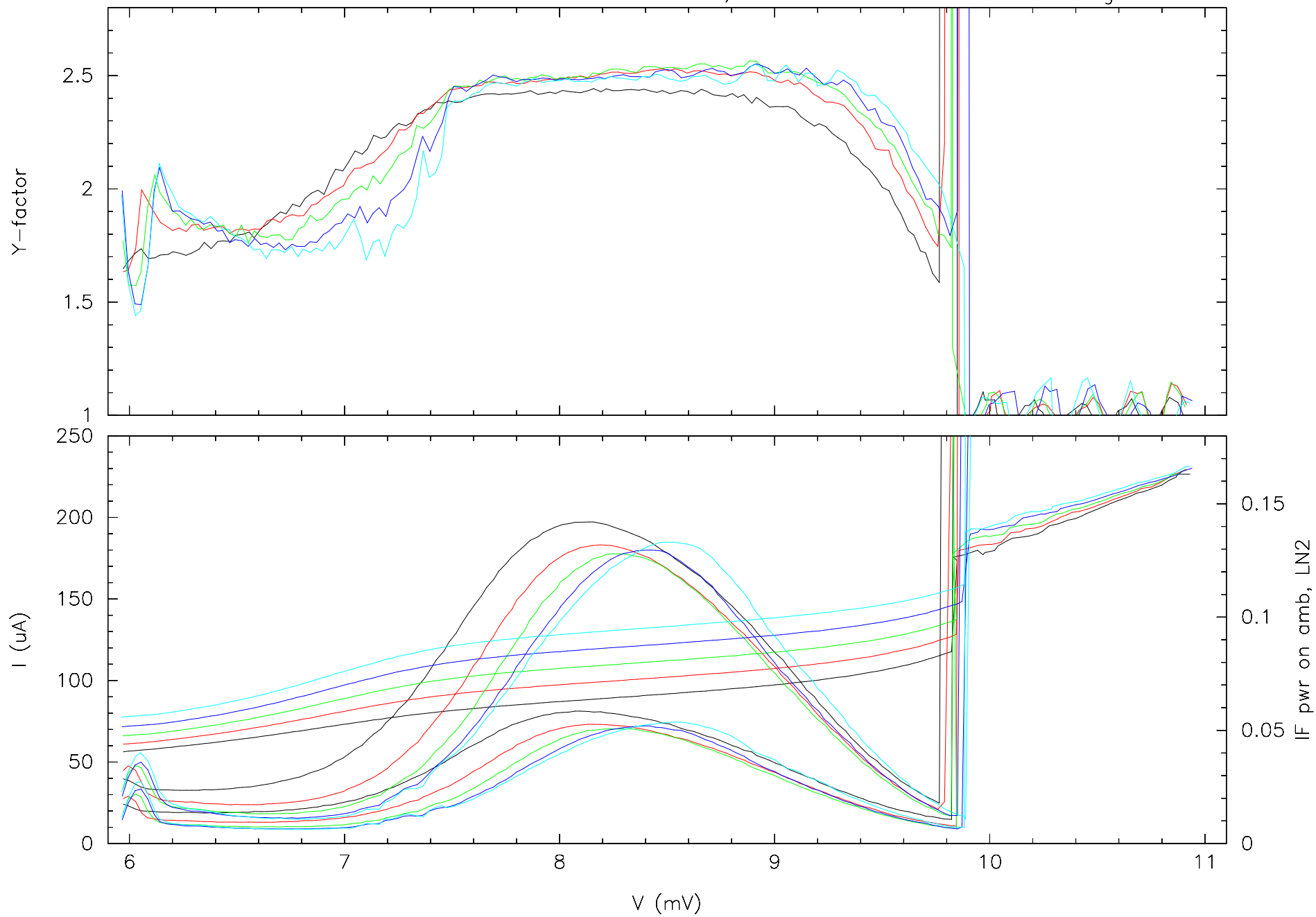
mixer 31-042-05; scans at 220 GHz with 135 mA magnet current
