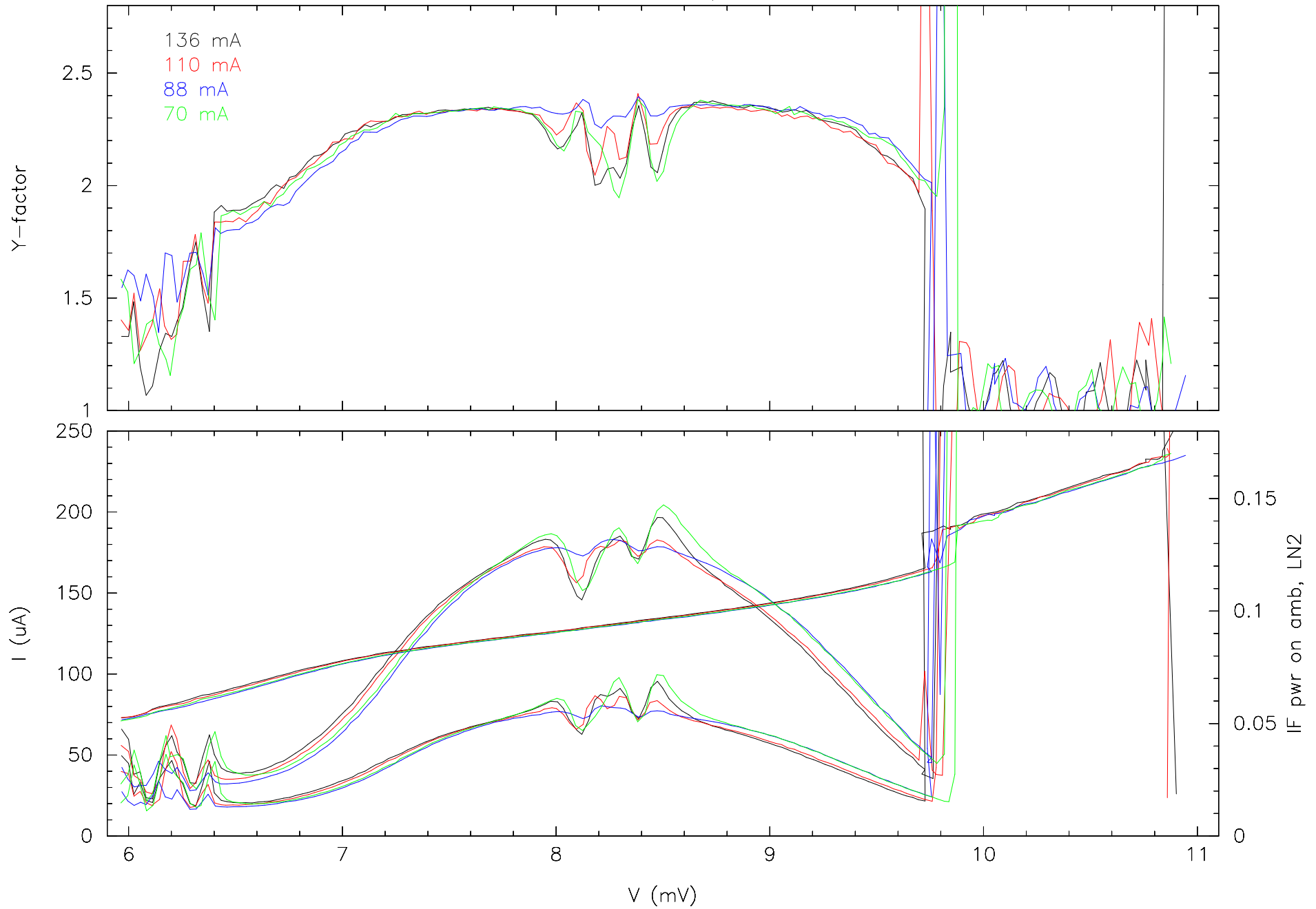
mixer 31-042-05; scans at 250 GHz with various solenoid currents
