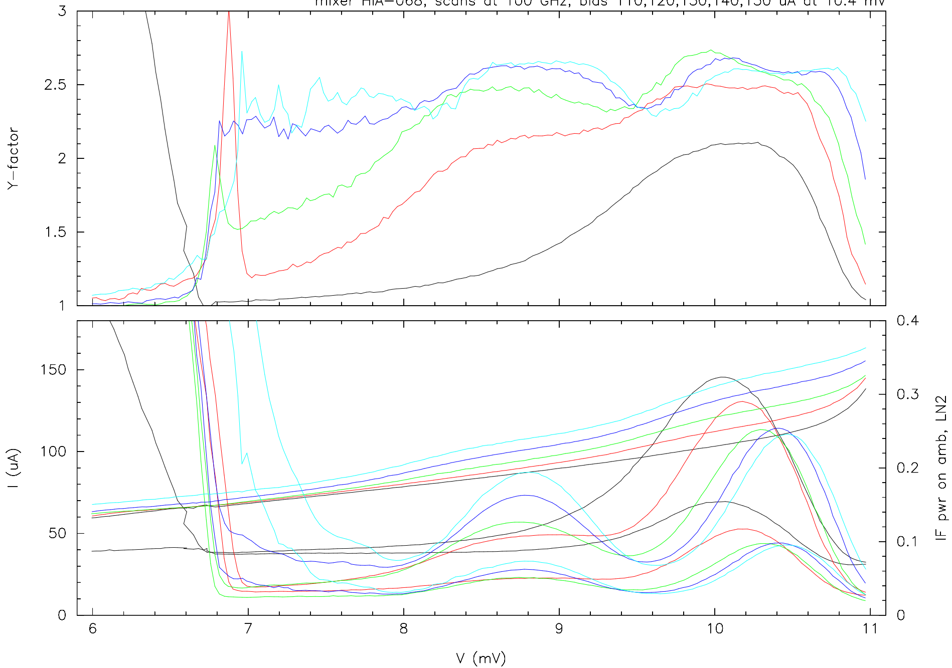
mixer HIA-068; scans at 100 GHz; bias 110,120,130,140,150 \mu\text{A} at 10.4 mV
