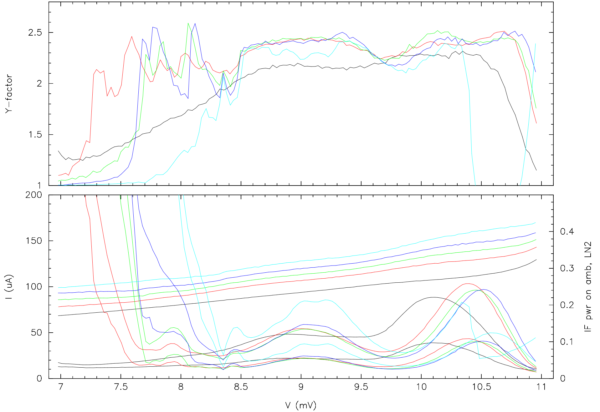
mixer HIA-073; scans at 90 GHz; bias 120,130,140,150,160 \mu\text{A}
