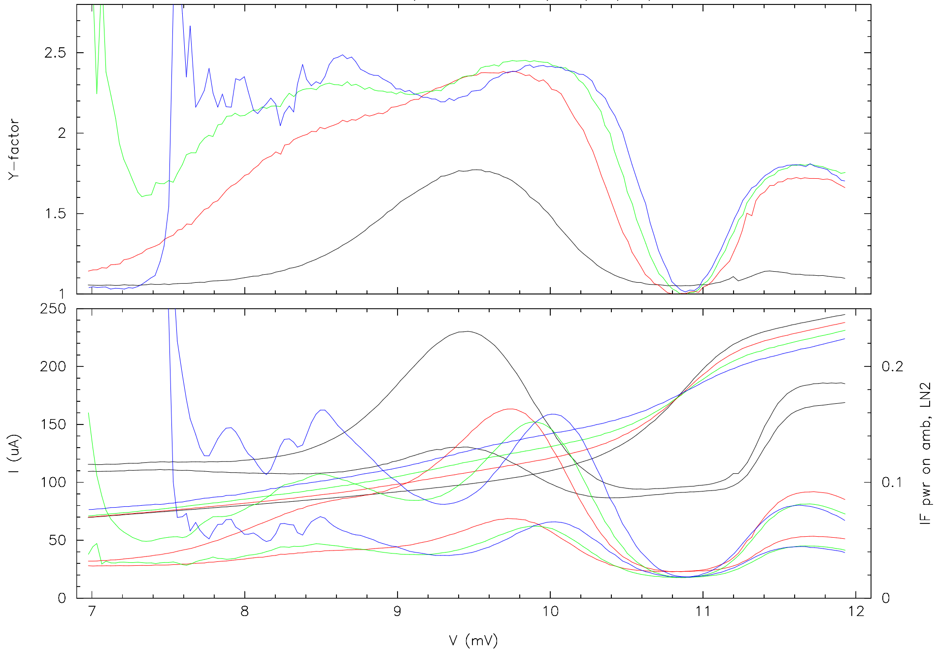
mixer HIA-091; scans at 90 GHz; 110,120,130,140 uA bias current at 10 mV
