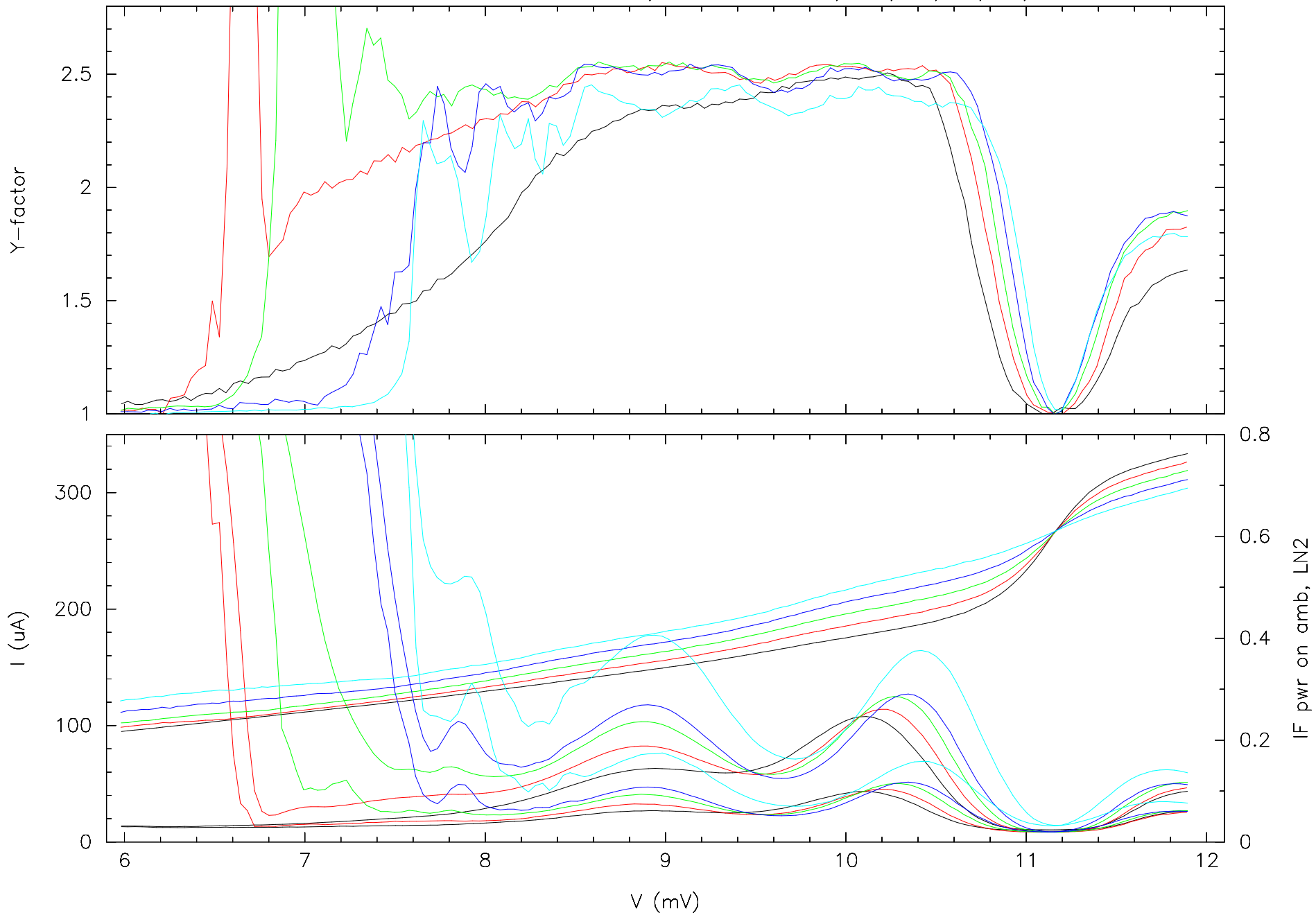
mixer HIA-180; scans at 90 GHz; 180,190,200,210,220 uA at 10.2 mV
