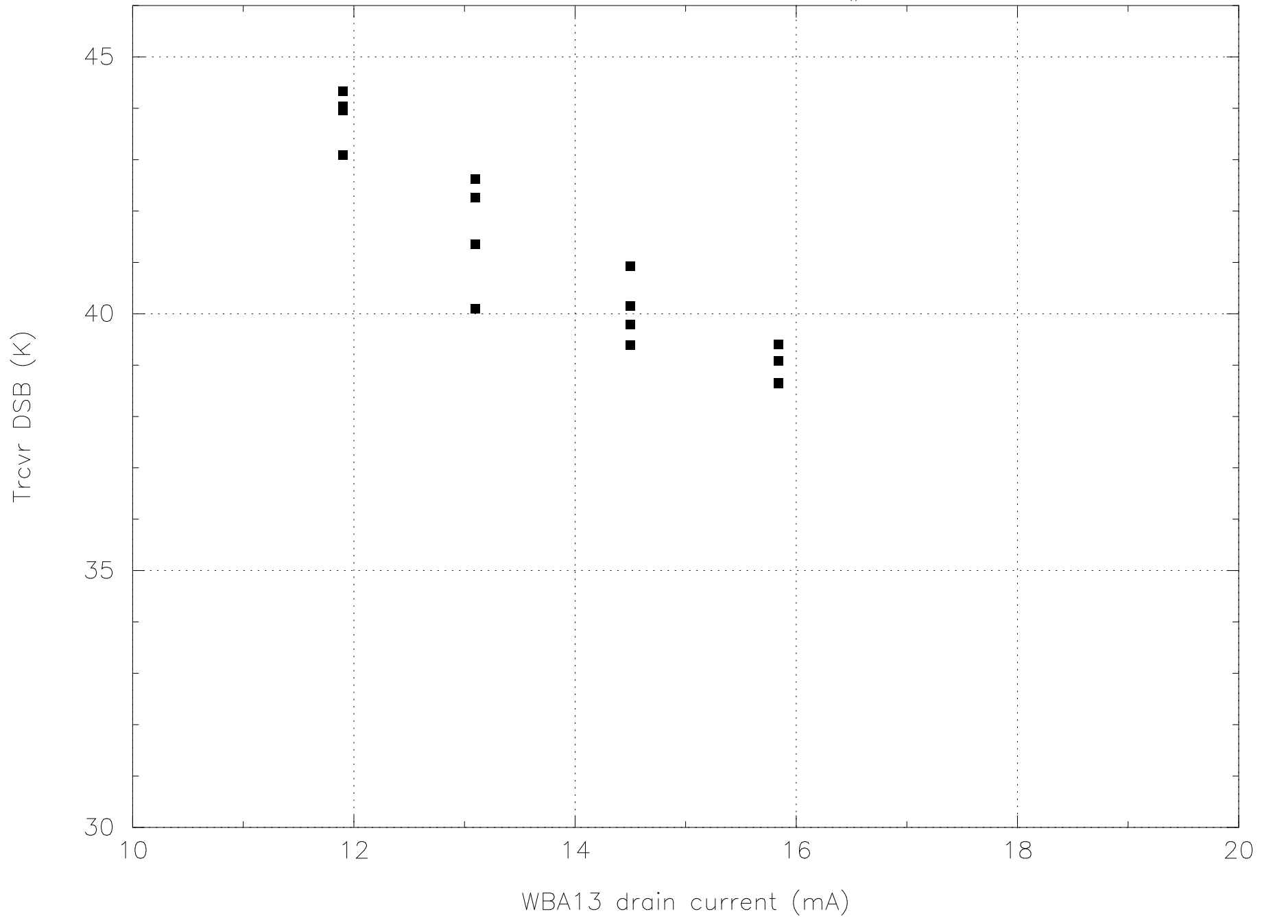
Trcvr vs drain current for HIA-181, WBA13 #15D, at 100 GHz
