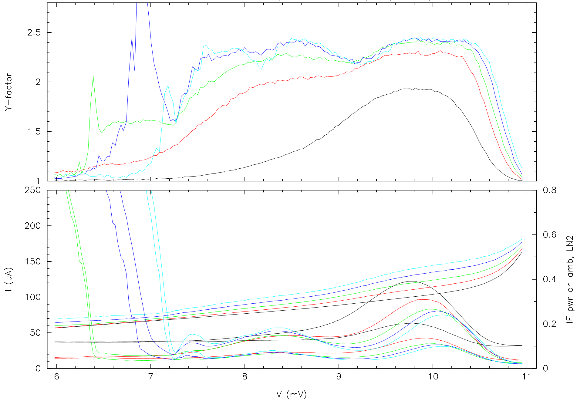
mixer HIA-181; scans at 110 GHz; 110,120,130,140,150 uA at 10.3 mV
