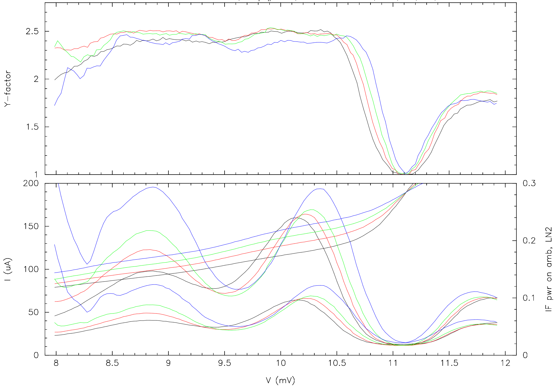
mixer HIA-185, amp #155D, scans at 90 GHz; 120,130,140,150 uA at 10.2 uA
