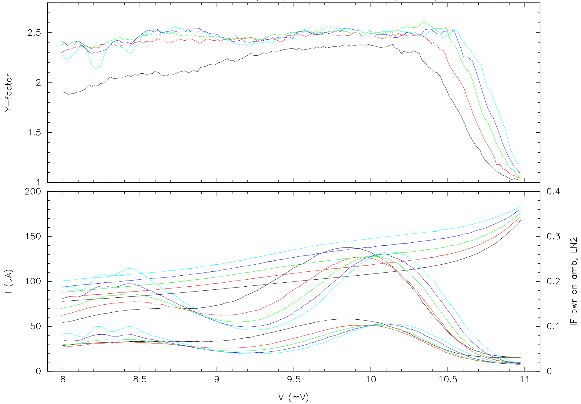
mixer HIA-188, amp #131D, scans at 110 GHz; 110,120,130,140,150 \mu\text{A} at 10.1 \mu\text{A}
