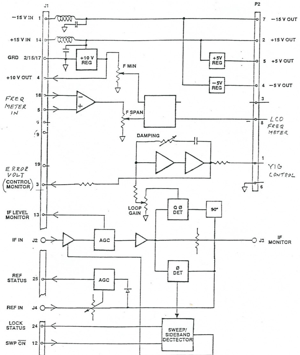
Figure 4. Block Diagram
