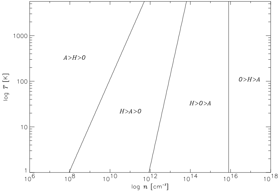
Figure 2: Parameter space for nonideal MHD. The curves correspond to the case v_A/c_S = 0.1 . (From Kunz & Balbus 2004, MNRAS, 348, 355.)
