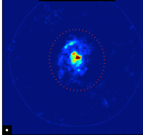
NGC5371
