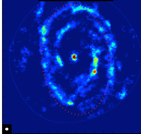
NGC6951
