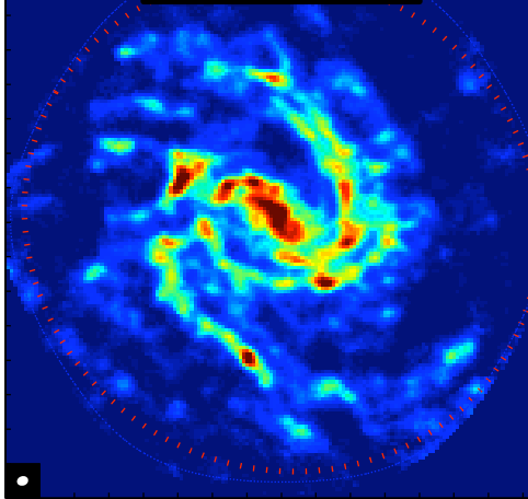
NGC4654
