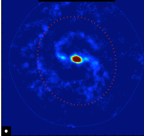
NGC4254
