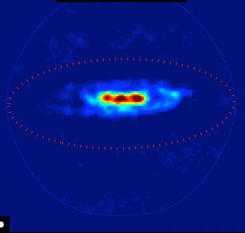
NGC4536
