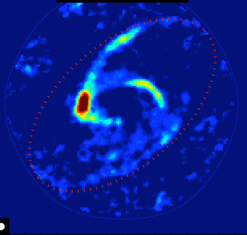
NGC3593
