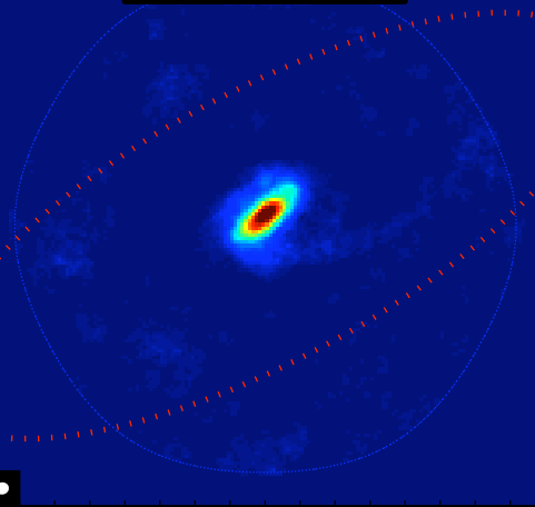
NGC5713
